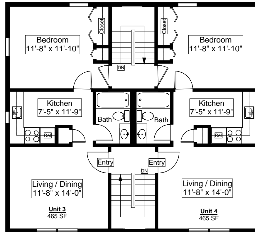
Second Floor Plan Ceiling Height = 7'-8"
