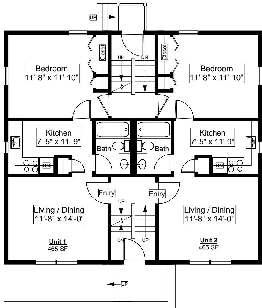
First Floor Plan Ceiling Height = 7'-8"
