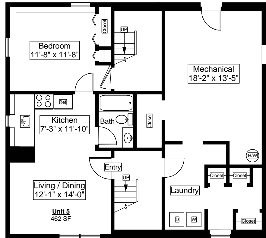
Lower Level Floor Plan Ceiling Height = 7'-2"
